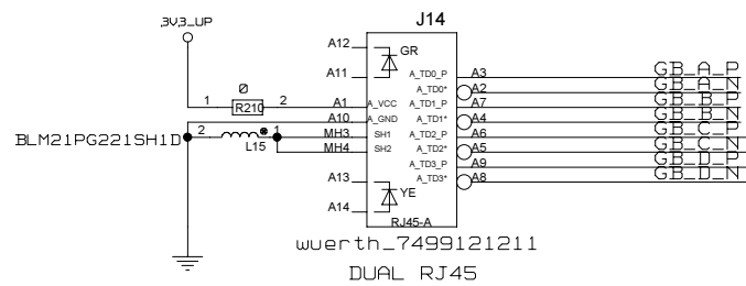
RJ45 FRONTPANEL
