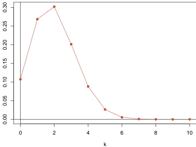
probabilities of bin( n=10, p=0.2 )
