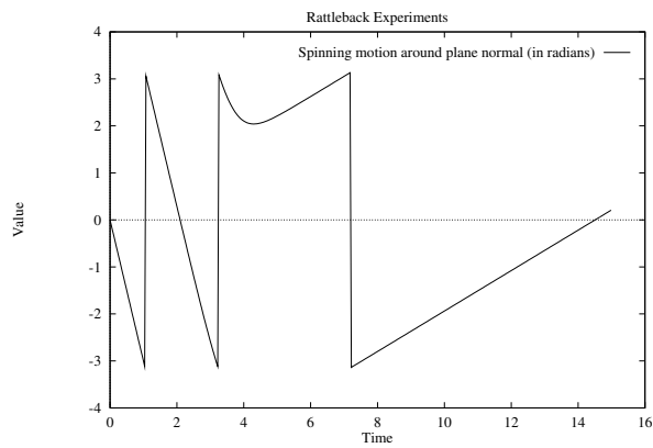
Figure 8: The reversion of the spin direction at time t \approx 4.5 described by the rotation of the rattleback about the plane-normal.
