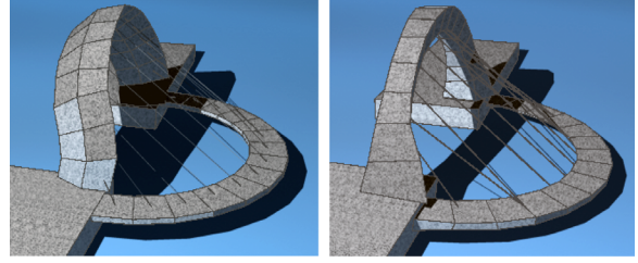
Figure 29: Improving the stability of a building using structural optimization, thus enabling a novel form-finding possibility [WSW*12].
