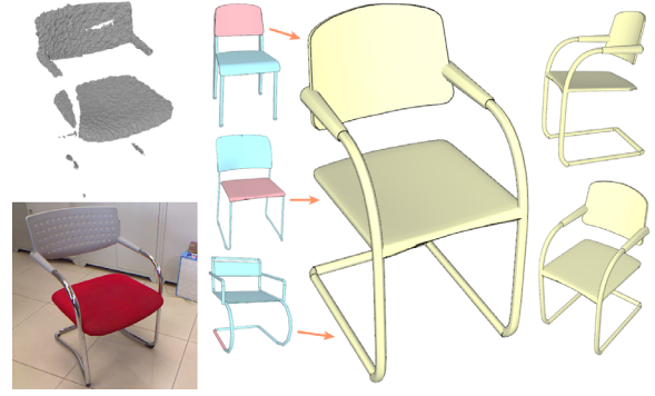
Figure 27: Structure-aware 3D model reconstruction from kinect data. The reconstruction is based on retrieving and then assembling parts taken from multiple example shapes in a small shape repository, while preserving the built-in structures of the examples [SFCH12].
