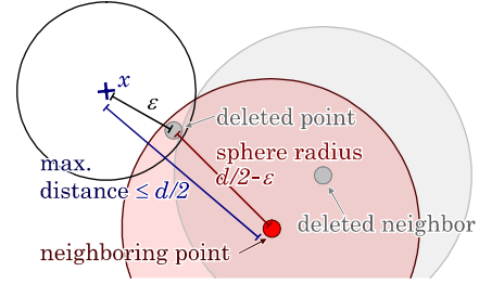
Figure 34: Stratification by removing points that are still covered by neighboring points.
