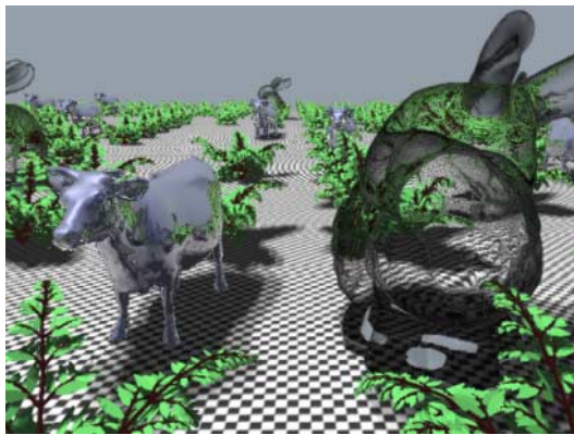
(c) point-based multi-resolution raytracing, 2×2 subpixel masks compositing (4062 sec.)
