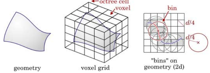
Figure 29: Dividing Geometry into bins. A grid divides the surface into fragments. Each fragment that contains a d/4 -interior point corresponds to a bin, i.e. it should receive at least one sample point. The right image shows the overlapping bins schematically in 2d.
