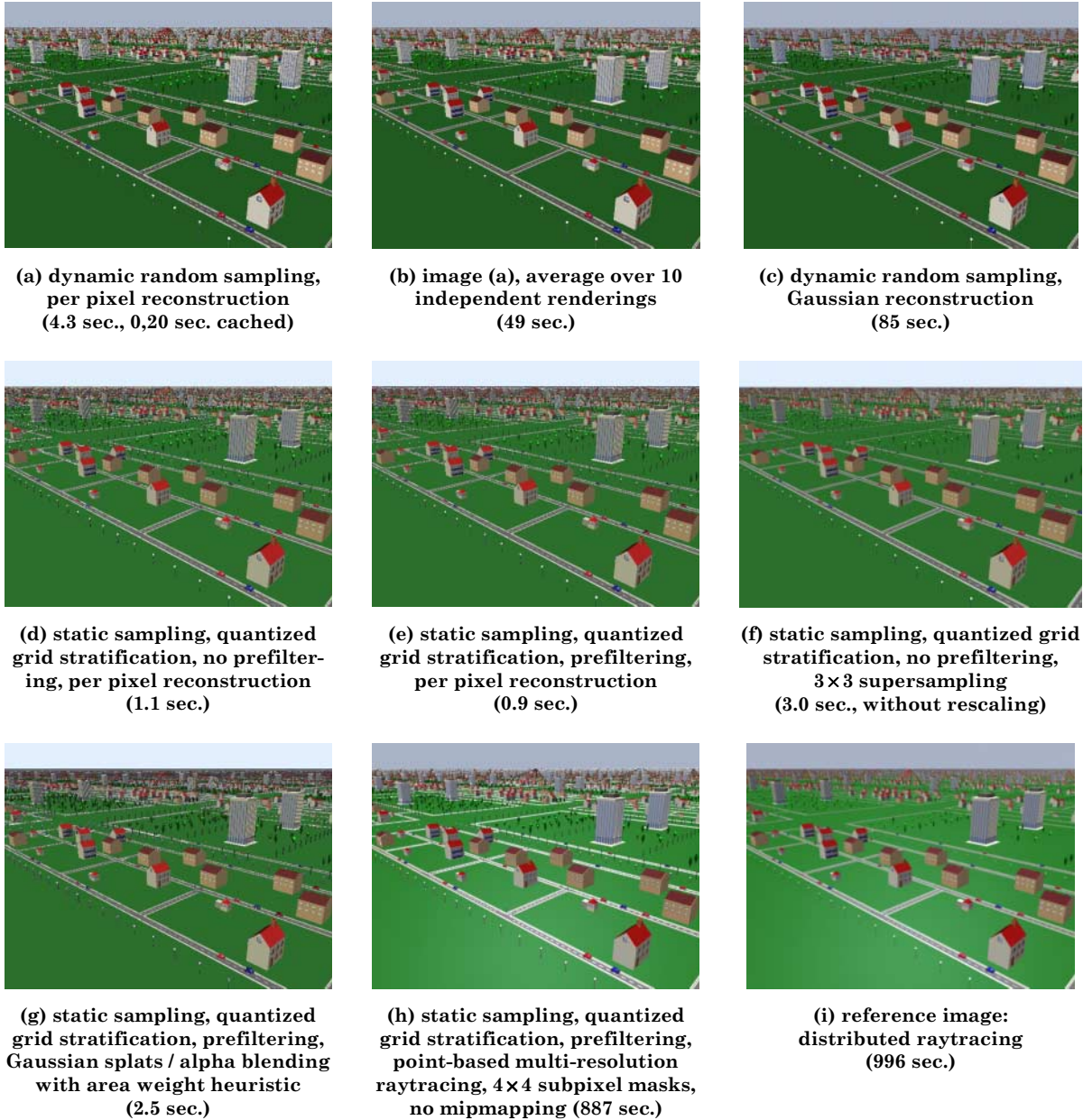
Figure 107: Image quality / antialiasing comparison for different image reconstruction techniques ( 640 \times 480 pixels). Scene: a city scene consisting of 192,431 triangles, replicated on two instantiation layers of 10 \times 10 instances each.
