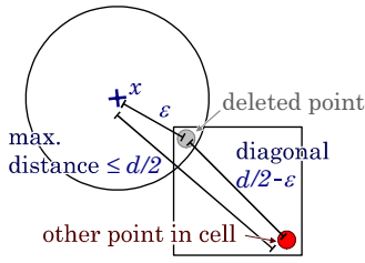
Figure 32: Grid stratification of random \varepsilon -sampling.
