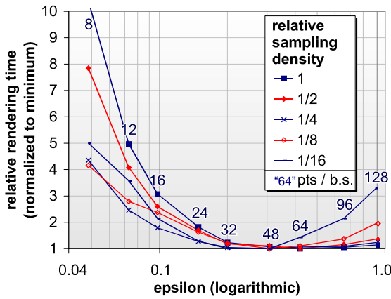
Figure 91: Trade-off between the rendering cost components for varying \varepsilon and different sampling densities. For static sampling, the optimal approximation accuracy is (roughly) the same for the different rendering resolutions (in contrast to dynamic sampling, see Figure 83)
