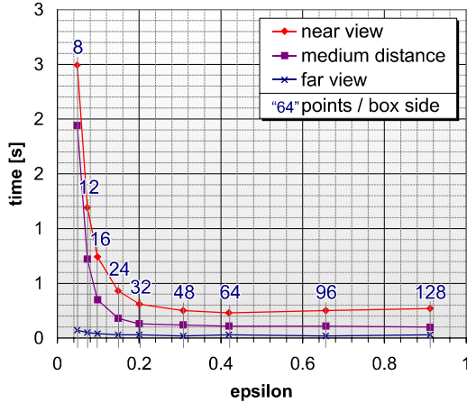
Figure 89: Rendering time (static sampling) for the scene depicted in Figure 79 in dependence of the approximation accuracy \varepsilon . For static sampling, much larger values of \varepsilon are favorable due to smaller point processing costs.
