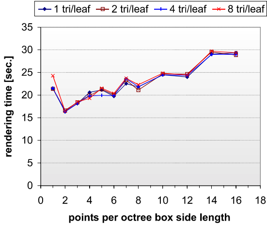
Figure 99: Rendering time for point-based multi-resolution raytracing (scene depicted in Figure 79a, near view) for a varying number of points per octree node and different numbers of triangles in leaf nodes. An optimal rendering time is achieved for k=2 points per box side length. The number of leaf node triangles has only a weak effect on the rendering time.
