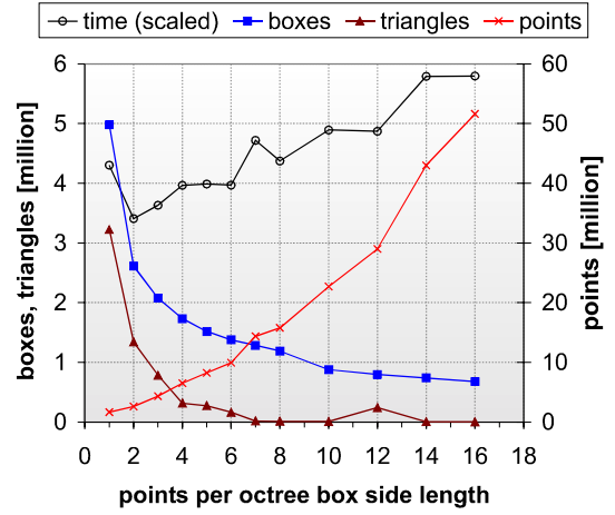
Figure 100: The number of points, triangles and boxes that have been tested for intersection by the point-based multi-resolution raytracing algorithm, in dependence of the number of points per octree box side length. Please note that the number of points is scaled differently (right caption) from the number of boxes and triangles (left caption).
