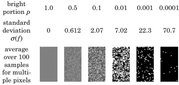
Figure 7: Monte Carlo integration ( n = 100 ) over multiple pixels in which a portion p of the pixel has a brightness of 1/(2p) (i.e. the correct result is \mu = 0.5 ). As the non-uniformity increases, the simple Monte Carlo approach becomes less efficient.
