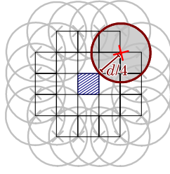
(a) 2d-case: at most 21 bins can overlap
