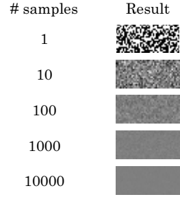
Figure 8: Monte Carlo integration over multiple pixels with varying sample size. Each pixel is half white and half black ( p = 0.5 , Figure 6b). Large sample sizes are needed to obtain a noise level below the level of perception.
