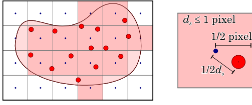
Figure 57: An on-screen sample spacing of d_s guarantees a safe coverage of closed surfaces.
