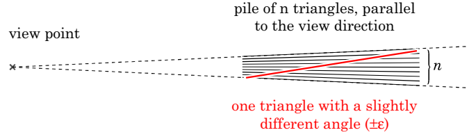
Figure 56: Worst case example for estimating the orientation factor. The projected area is overestimated by an arbitrary factor.
