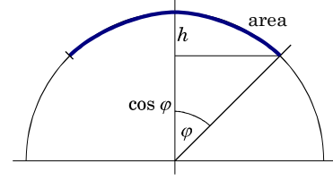
Figure 54: Area on the unit sphere in dependence of the angle \phi
