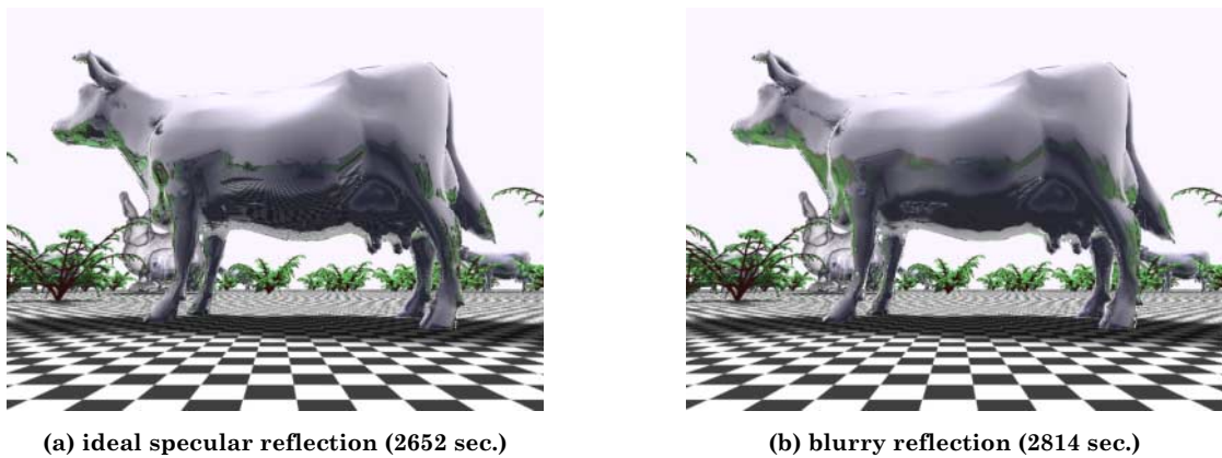
Figure 119: Blurry Reflections in a more complex scene (cf. Figure 113, 640×480 pixels). In the left image, it can be seen nicely that linearly interpolated normals lead to piecewise constant second derivatives, i.e. constant footprint increments and thus a constant resampling filter on each triangle. In the right image, the ray footprint increments have been increased to simulate blurry reflections.
