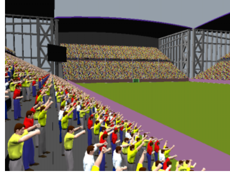
(b) near view (1.7M points, 585K triangles, 3641 nodes, 9.3fps)
