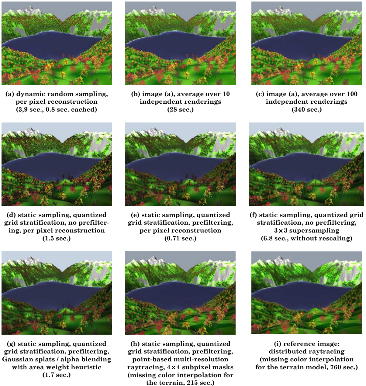
Figure 105: Image quality / antialiasing comparison for different image reconstruction techniques (640×480 pixels). Scene: replicated trees, near view (16×16, 2 hierarchy layers, cf. Figure 79)
