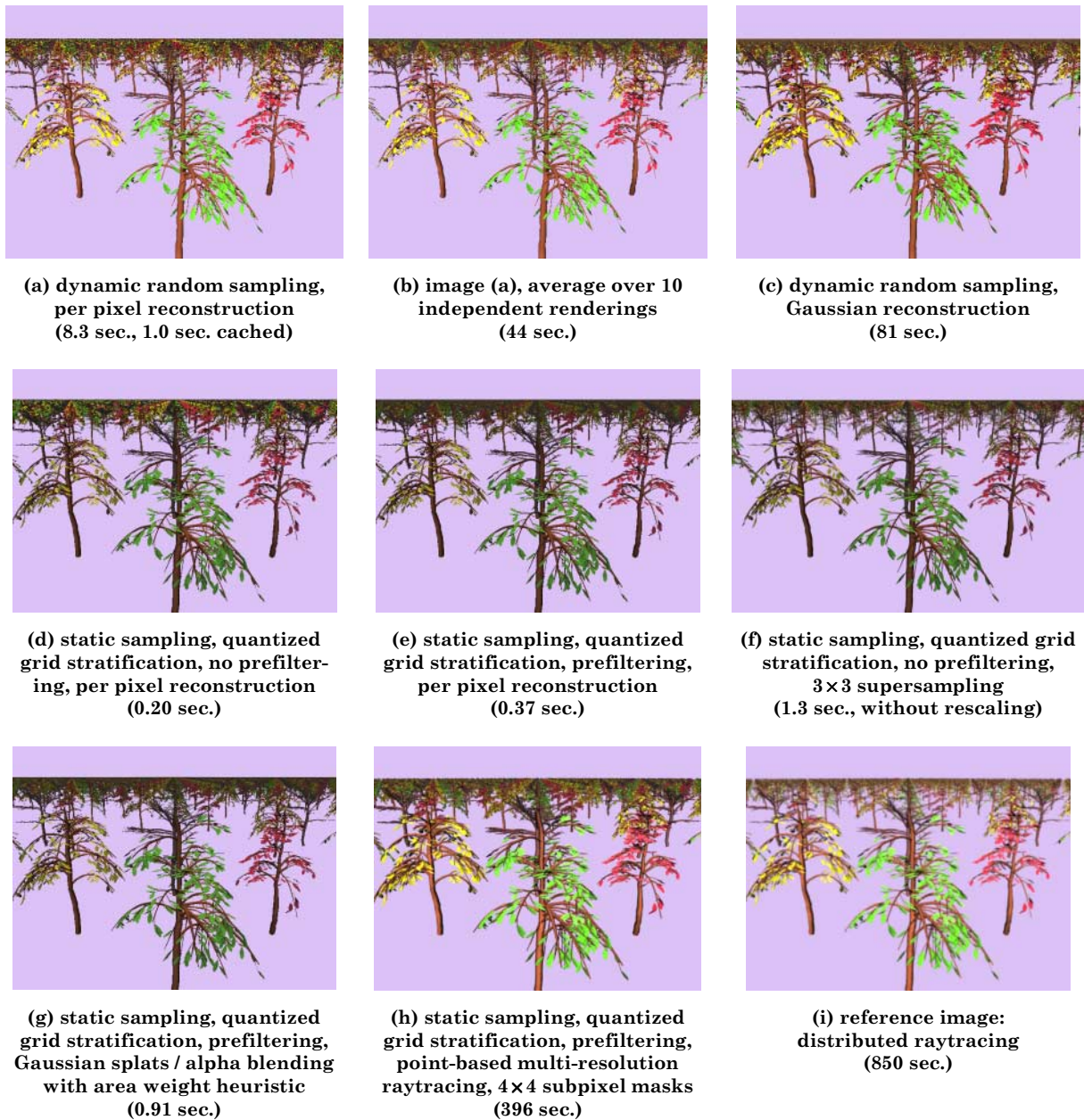
Figure 104: Image quality / antialiasing comparison for different image reconstruction techniques ( 640 \times 480 pixels). Scene: replicated trees, near view ( 16 \times 16 , 2 hierarchy layers, cf. Figure 79)
