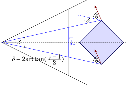
Figure 55: Orientational deviation due to spatial deviation.
