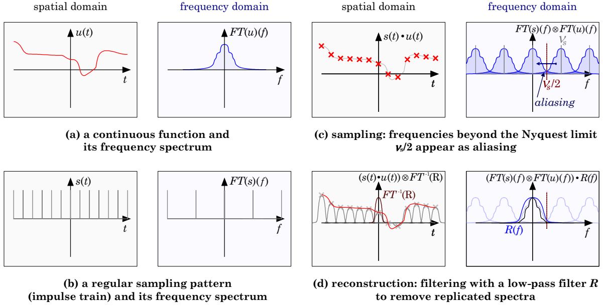
Figure 5: Explanation of the aliasing phenomenon in frequency space [Foley et al. 96].
