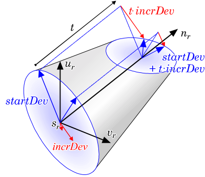
Figure 64: Ray coordinates.
