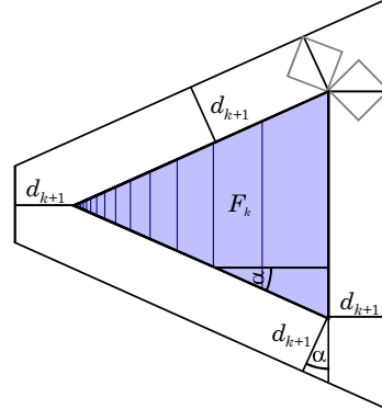
Figure 50: Cumulative depth regions F_k := \bigcup_{i=1..k} (\text{region } k) , extended by d_{k+1} .
