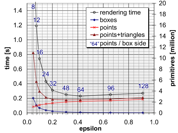
Figure 90: Number of processed primitives for varying approximation accuracies \varepsilon (scene: Figure 79, near view). Again, the number of sample points grows for larger \varepsilon while the number of hierarchy nodes and triangles grows for small \varepsilon .
