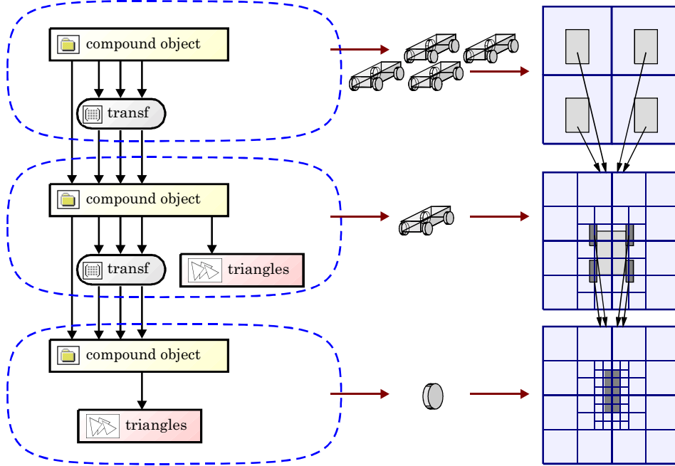
Figure 26: Scene graph based instantiation combined with spatial data structures for efficient sample point extraction. Spatial data structures can be assigned to groups of objects. A complete data structure is treated as compound object and inserted into a parent data structure. During traversal, the instantiation transforms have to be considered to retain the impression of one “large” octree.
