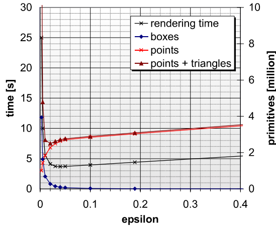
Figure 81: The number of processed primitives for varying approximation accuracies \epsilon (near view). For small \epsilon processing the boxes and box-exceeding triangles dominates the rendering costs, for large \epsilon the costs are dominated by processing sample points.
