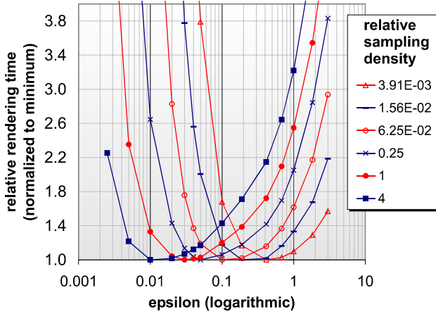
Figure 83: Trade-off between the rendering cost components for varying \epsilon and different sampling densities. The larger the number of sample points per box, the smaller is the optimal approximation accuracy \epsilon .
