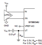
Figure 3c. LVPECL Interface (DC-Coupled)
