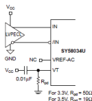
Figure 3c. LVPECL Interface (DC-Coupled)
