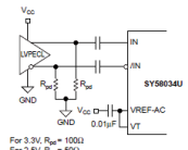
Figure 3d. LVPECL Interface (AC-Coupled)
