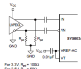
Figure 3d. LVPECL Interface (AC-Coupled)
