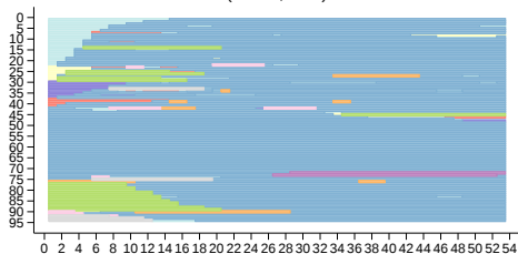
Cluster 1 (n = 94, 44%)
