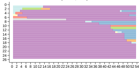
Cluster 2 (n = 25, 12%)
