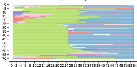
Cluster 3 (n = 70, 32%)
