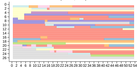
Cluster 4 (n = 26, 12%)
