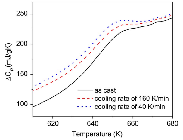
FIG. 4. (Color online) The curves of the DSC obtained from the as-cast and quenched \text{Zr}_{46.75}\text{Ti}_{8.25}\text{Cu}_{7.5}\text{Ni}_{10}\text{Be}_{27.5} (Vit4) BMGs. The quenching process involves the heating up to 713 K at a heating rate of 40 K/min and the cooling down to room temperature at cooling rates of 160 and 40 K/min, respectively.
