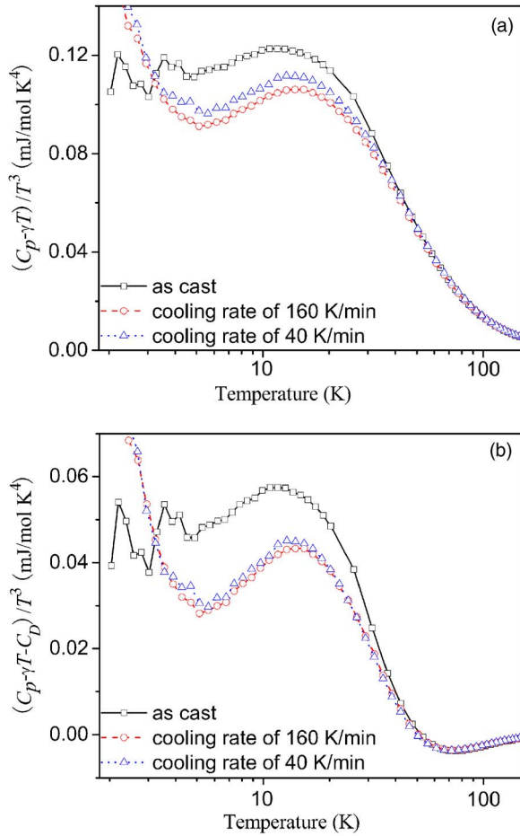
FIG. 5. (Color online) The (C_p - \gamma T)/T^3 (a) and (C_p - \gamma T - C_D)/T^3 (b) vs T plots of the as-cast and quenched vit4 BMGs. The quenching process involves the heating up to 713 K at a heating rate of 40 K/min and the cooling down to room temperature at cooling rates of 160 and 40 K/min, respectively.
