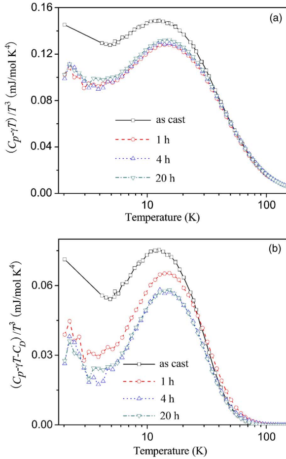
FIG. 3. (Color online) The (C_p - \gamma T)/T^3 (a) and (C_p - \gamma T - C_D)/T^3 (b) vs T plots of the as-cast and annealed (\text{Cu}_{50}\text{Zr}_{50})_{92}\text{Al}_8 BMGs. The annealing of (\text{Cu}_{50}\text{Zr}_{50})_{92}\text{Al}_8 BMGs was performed at 673 K below the calorimetric glass transition temperature (701 K) for 1, 4, and 20 h.
