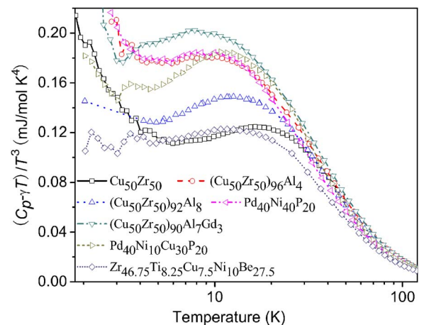
FIG. 1. (Color online) The (C_p - \gamma T)/T^3 vs T plots of our measured representative BMGs after subtracting the electronic and/or magnetic contributions.
