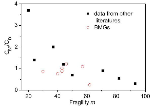
FIG. 2. (Color online) The ratio of the BP to the Debye contributions around the maximum vs the fragility m of our measured BMGs and some traditional glasses collected from literatures. The data are also listed in Table II.
