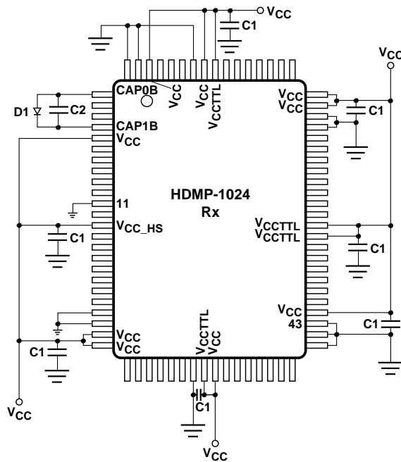
Figure 20b. HDMP-1022 (Rx) Power Supply Bypass.
