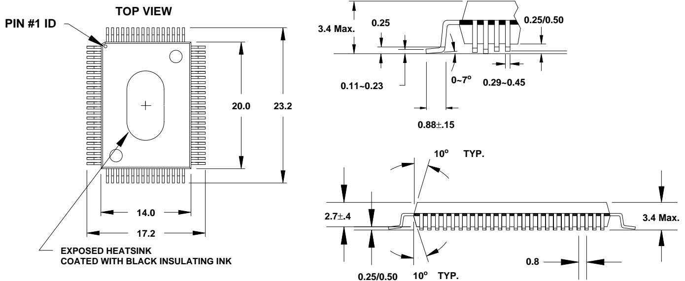
Figure 10. Mechanical Dimensions of HDMP-1022 and HDMP-1024.
