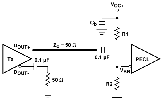
D) SINGLE-ENDED DRIVE TO A PECL INPUT
