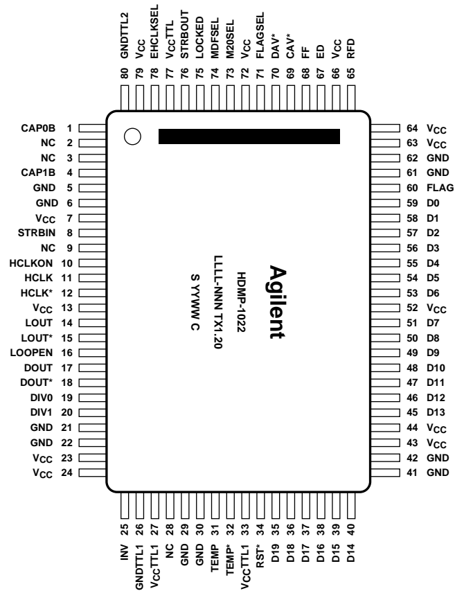
Figure 8. HDMP-1022 (Tx) Package Layout, Top View.
