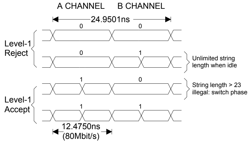
Figure 3 TDM biphasemark encoding
