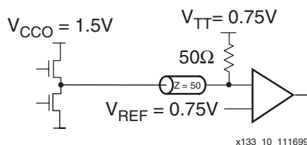
Figure 2-87: Terminated HSTL Class I
