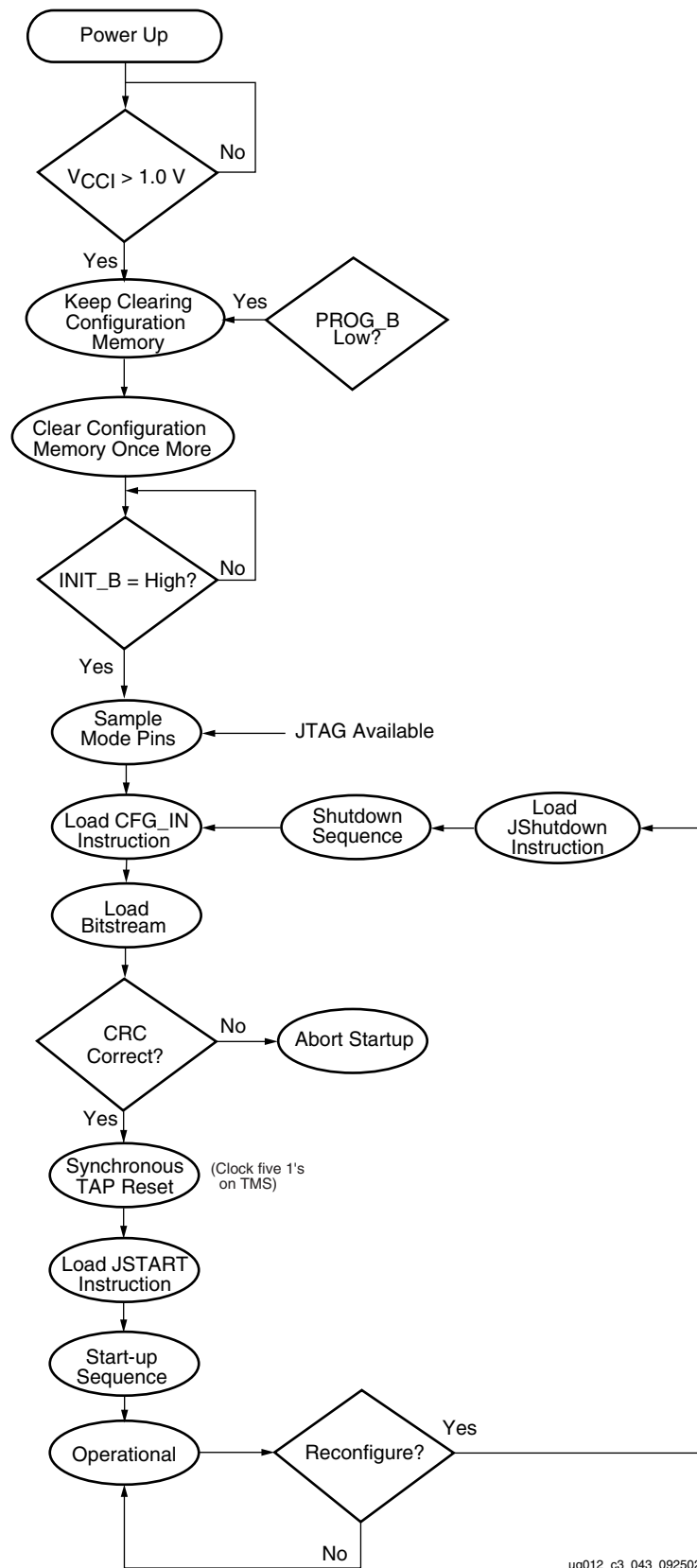
Figure 3-26: Device Configuration Flow Diagram
