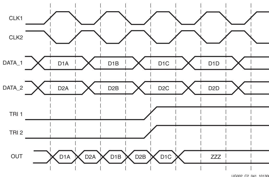
Figure 2-117: Timing Diagram for Output DDR With 3-State Control
