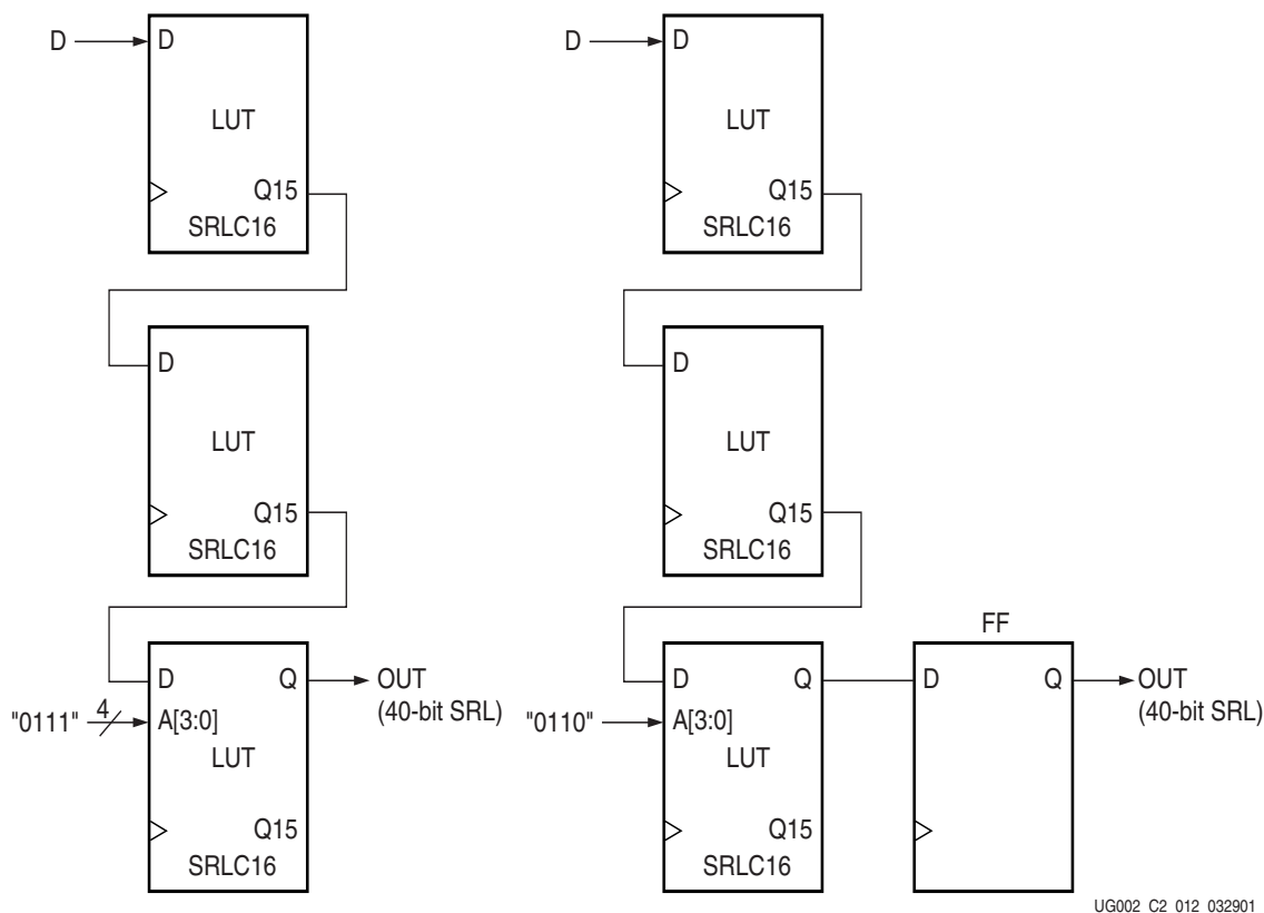
Figure 2-63: 40-bit Static-Length Shift Register
