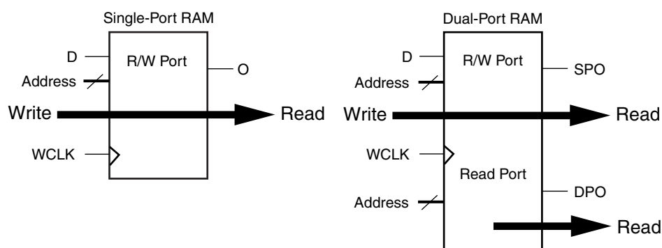
Figure 2-52: Single-Port and Dual-Port Distributed SelectRAM
