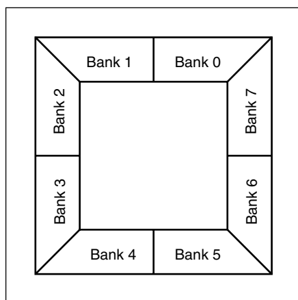
Figure 2-79: Virtex-II I/O Banks: Top View for Flip-Chip Packages (FF & BF)
