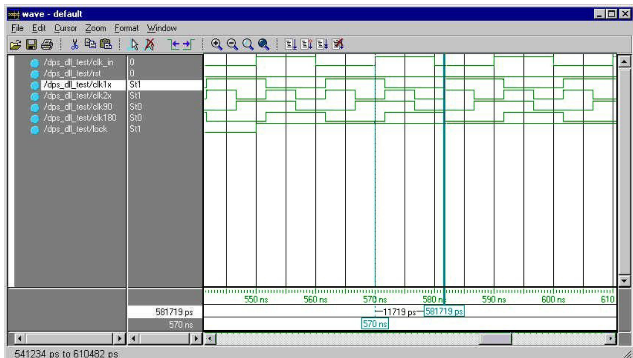
Figure 2-43: DCM_DPS Waveforms
