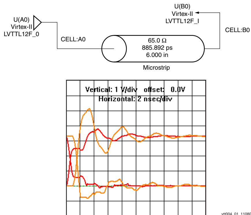
Figure 4-69: Unterminated Example
