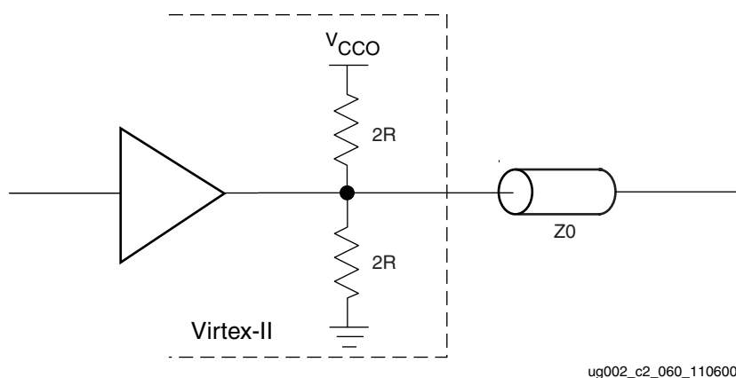
Figure 2-108: Driver With Split Termination Using DCI
