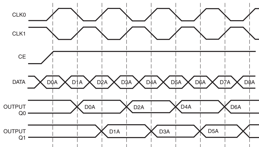
Figure 2-113: Input DDR Timing Diagram
