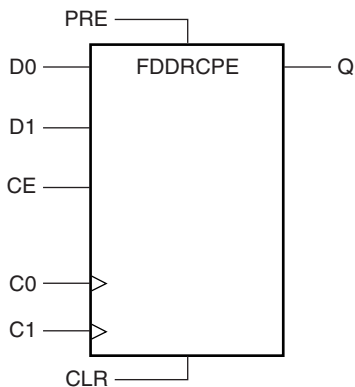
Figure 2-119: FDDRCPE Symbol: DDR Flip-Flop With Clock Enable and Asynchronous PRESET and CLR
