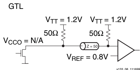
Figure 2-85: GTL Terminated
