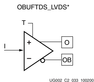
Figure 2-124: LVDS 3-State Primitives
