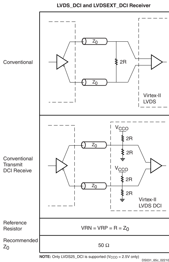
Figure 2-111: LVDS DCI Usage Examples
