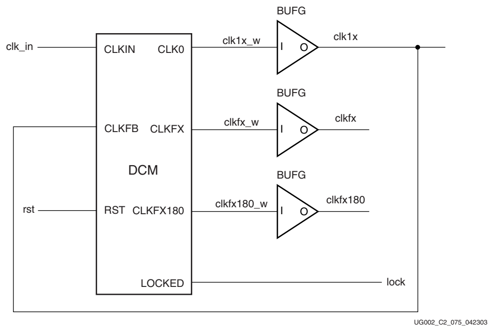
Figure 2-31: BUFG_DFS_FB_SUBM
