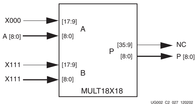
Figure 2-76: TWOS_CMP9 Submodule
