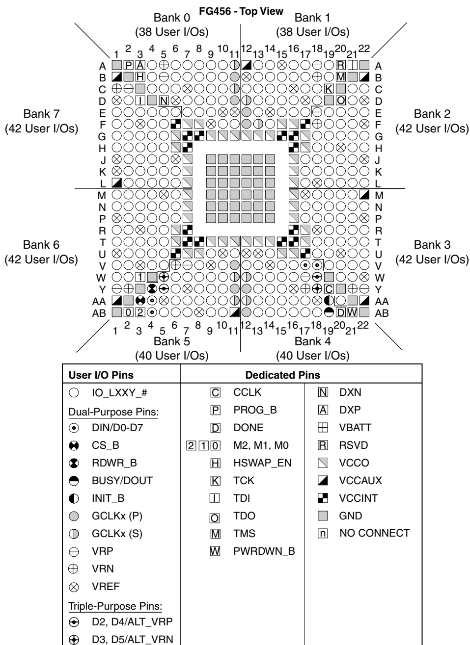
Figure 4-5: FG456 Fine-Pitch BGA Composite Pinout Diagram (XC2V1000)
