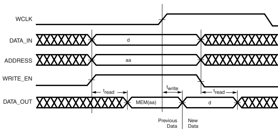
Figure 2-53: Write Timing Diagram
