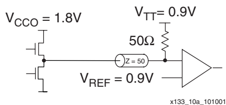
Figure 2-91: Terminated HSTL Class I (1.8V)
