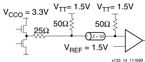
Figure 2-96: Terminated SSTL3_II
