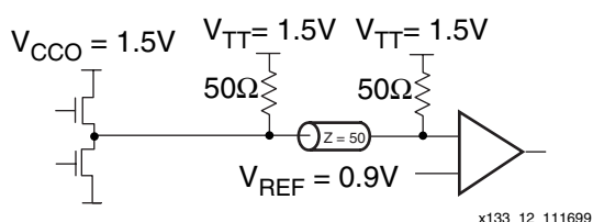
Figure 2-90: Terminated HSTL Class IV
