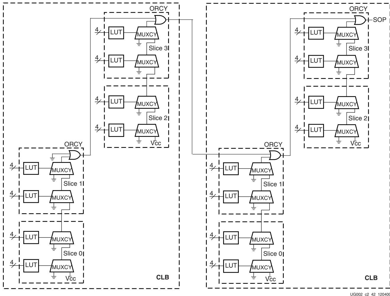
Figure 2-71: 64-bit Input SOP Design
