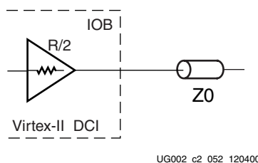
Figure 2-100: Controlled Impedance Driver With Half Impedance
