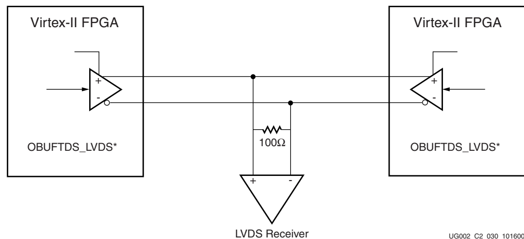
Figure 2-125: LVDS 3-State Termination
