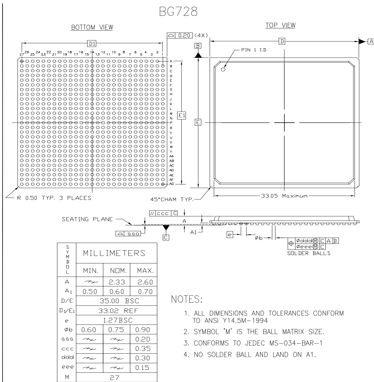
Figure 4-36: BG728 Standard BGA Package
