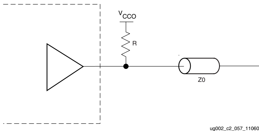
Figure 2-105: Driver With Single Termination Without DCI
