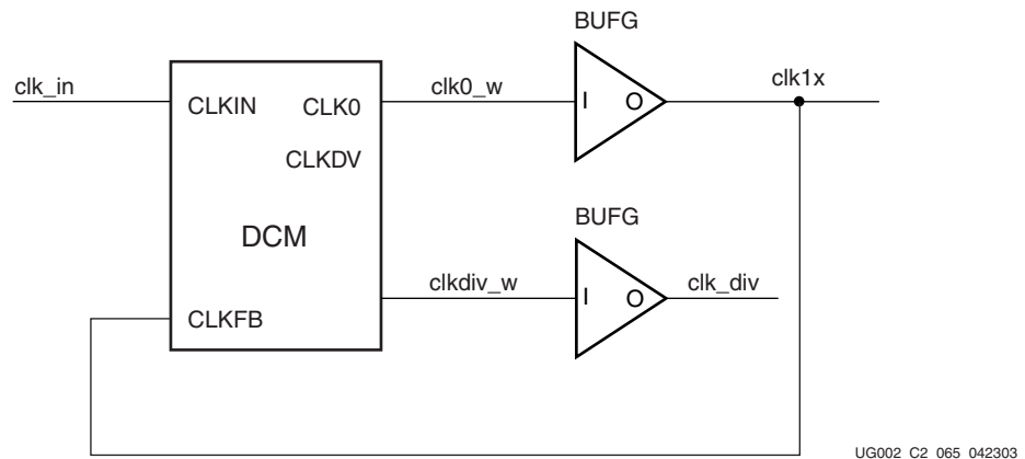
Figure 2-28: BUFG_CLKDV_SUBM
