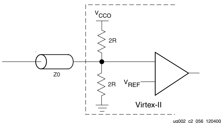
Figure 2-104: Split Termination Using DCI
