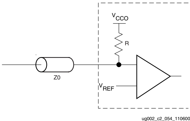
Figure 2-102: Single Termination Using DCI
