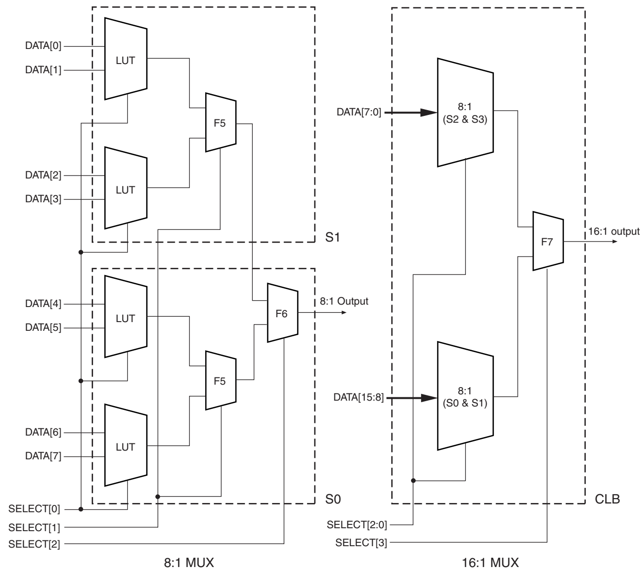
Figure 2-69: 8:1 and 16:1 Multiplexers
