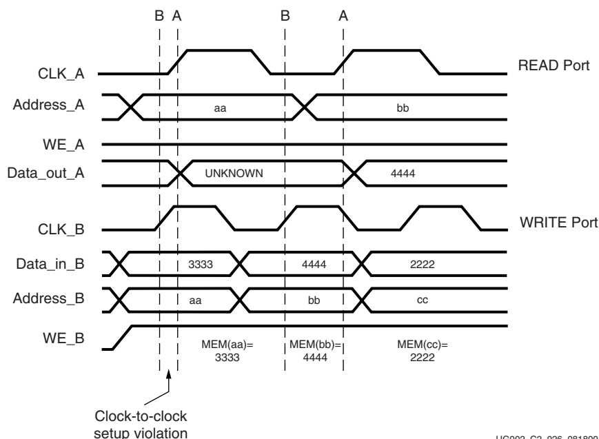
Figure 2-49: READ-WRITE Conditions
