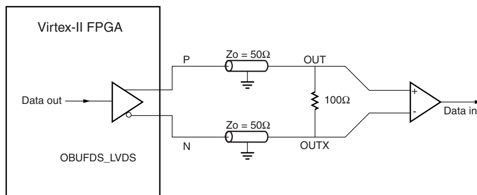
Figure 2-123: LVDS Transmitter Termination
