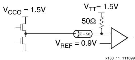
Figure 2-89: Terminated HSTL Class III
