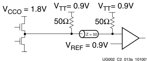
Figure 2-92: Terminated HSTL Class II (1.8V)
