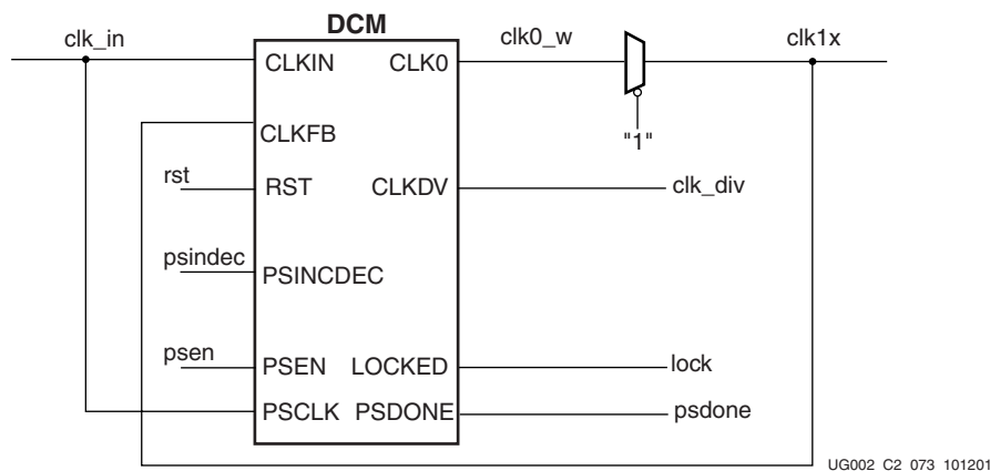
Figure 2-40: BUFG_PHASE_CLKDV_SUBM
