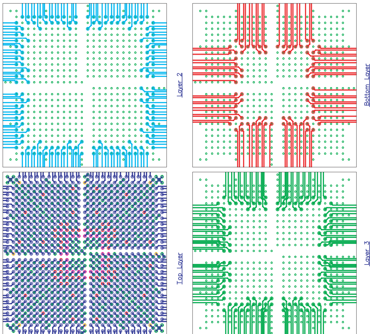
Figure 4-58: BG728 Standard Routing
