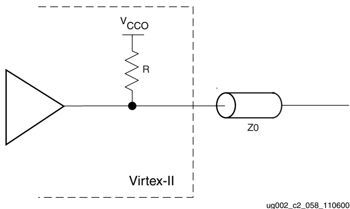
Figure 2-106: Driver With Single Termination Using DCI
