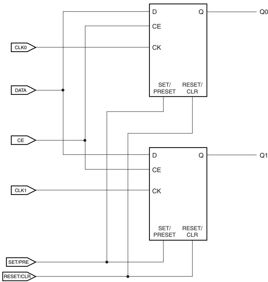
Figure 2-112: Input DDR
