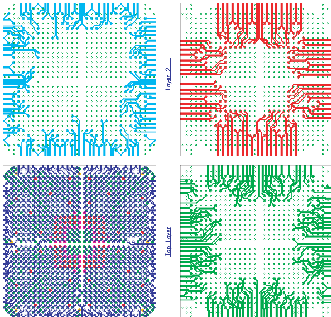
Figure 4-67: BF957 Routing With LVDS Pairs
