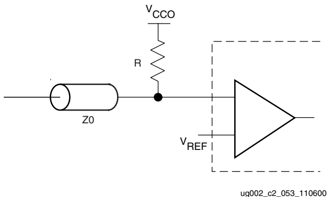
Figure 2-101: Single Termination Without DCI
