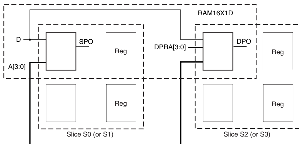
Figure 2-55: RAM16X1D Placement
