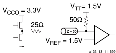
Figure 2-95: Terminated SSTL3_I
