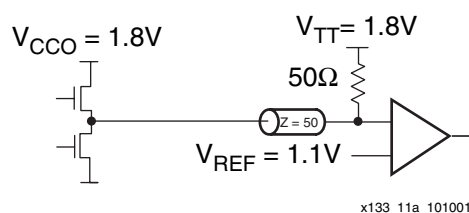
Figure 2-93: Terminated HSTL Class III (1.8V)
