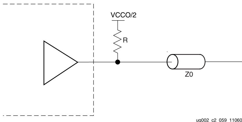
Figure 2-107: Driver With Split Terminating
