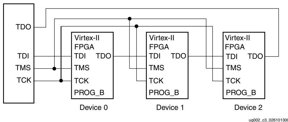
Figure 3-27: Boundary Scan Chain of Devices
