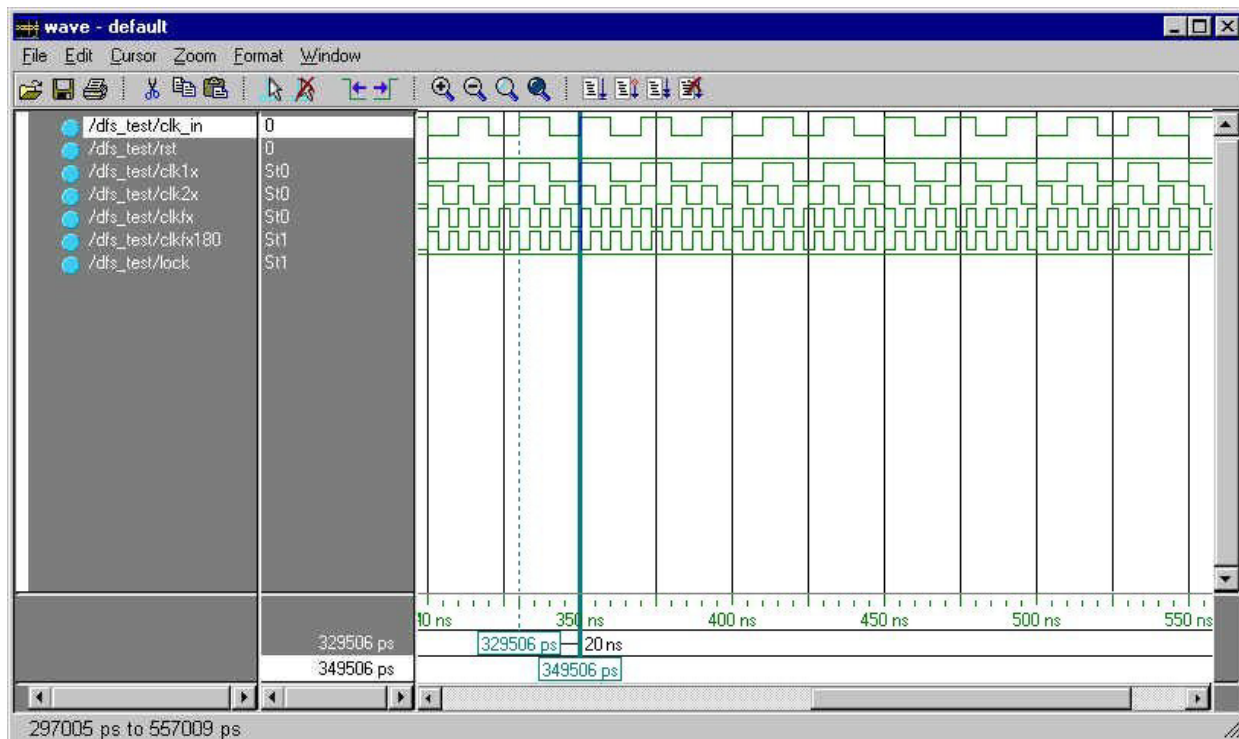
Figure 2-42: DCM_DFS Waveforms
