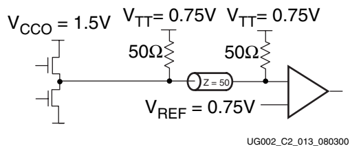
Figure 2-88: Terminated HSTL Class II
