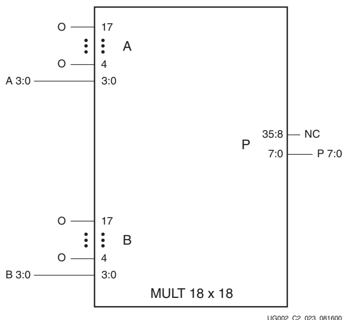
Figure 2-75: MULT4X4_U Submodule
