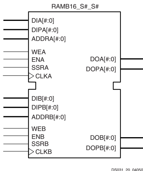
Figure 2-50: Dual-Port Block RAM Primitive
