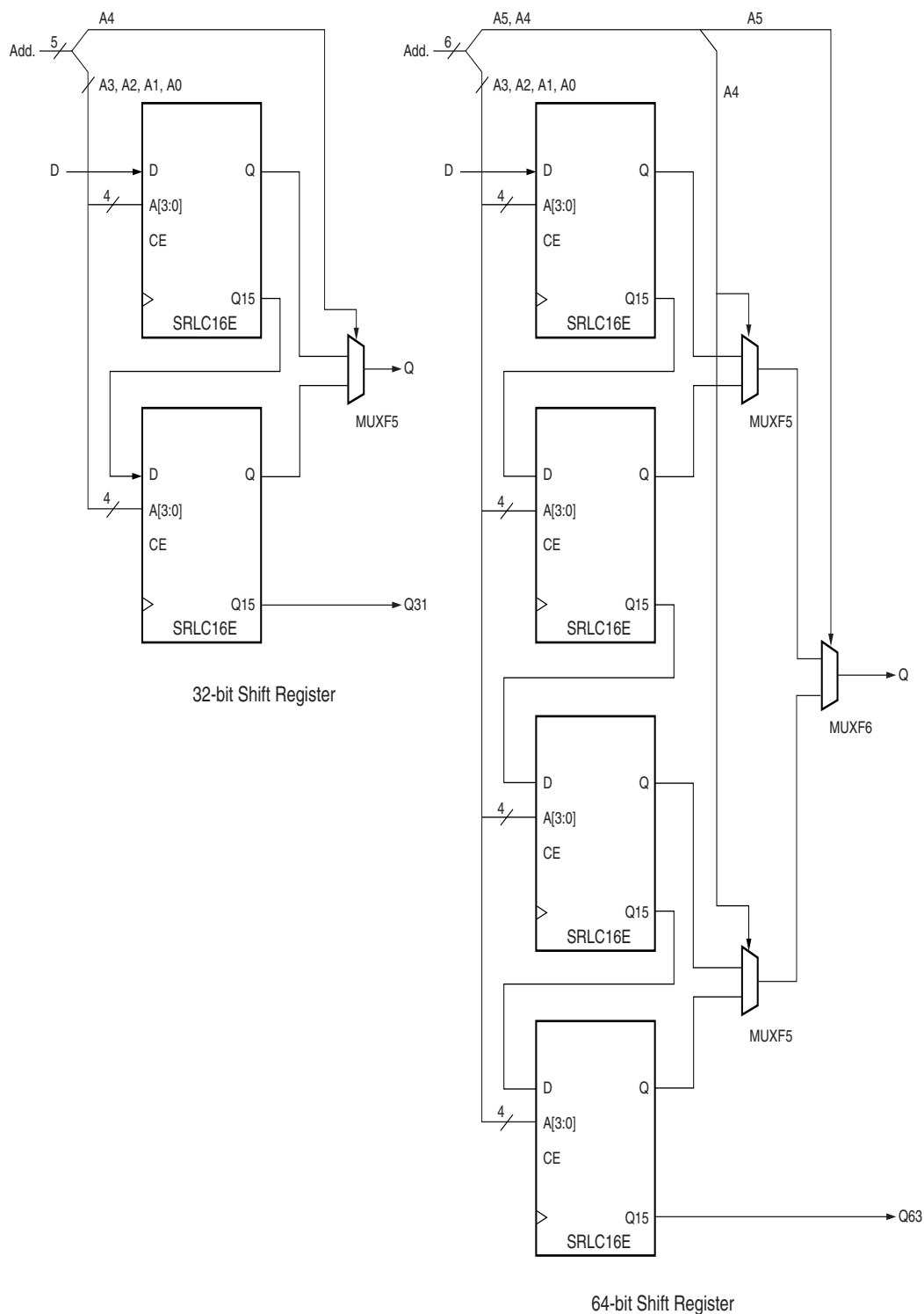
Figure 2-60: Shift-Register Submodules (32-bit, 64-bit)
