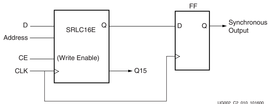
Figure 2-62: Fully Synchronous Shift Register
