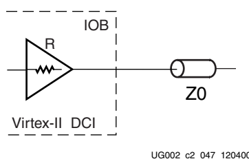
Figure 2-99: Controlled Impedance Driver
