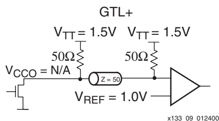
Figure 2-86: GTL+ Terminated
