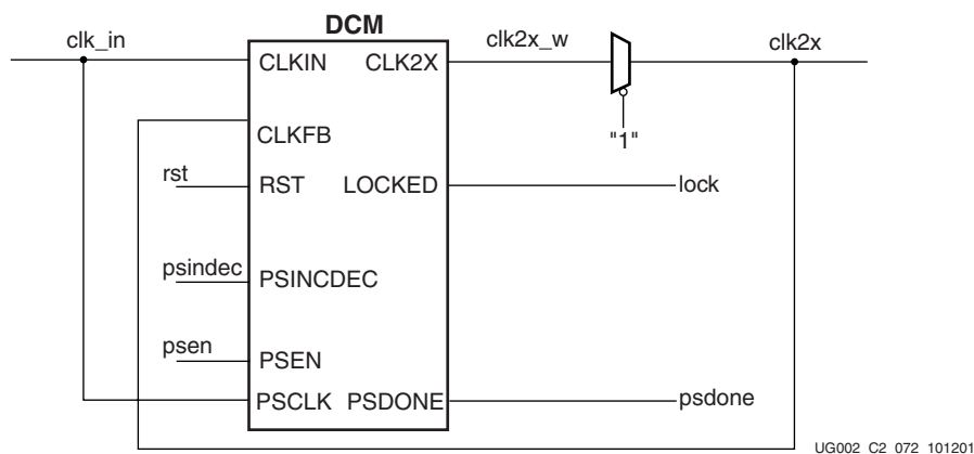
Figure 2-39: BUFG_PHASE_CLK2X_SUBM
