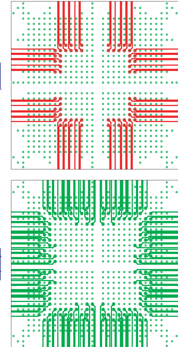
Figure 4-66: BF957 Standard Routing
