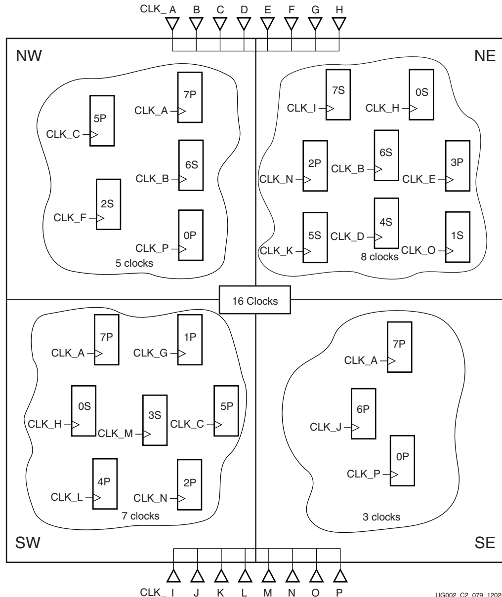
Figure 2-12: 16-Clock Floorplan
