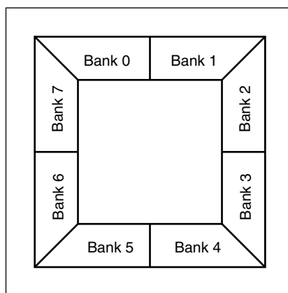
Figure 2-80: Virtex-II I/O Banks: Top View for Wire-Bond Packages (CS, FG, & BG)
