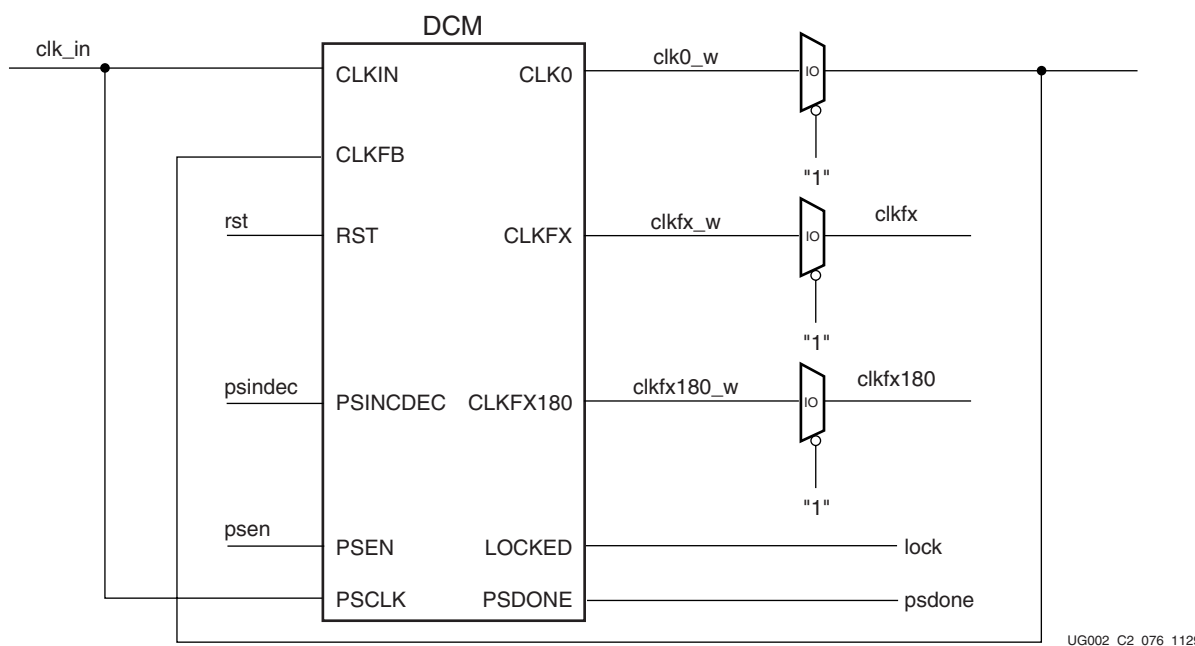
Figure 2-38: BUFG_PHASE_CLKFX_FB_SUBM
